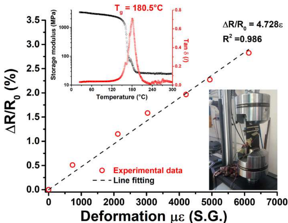
Fig. 3. Piezoresistive characterization in tensile tests of coated CFRP specimen.
